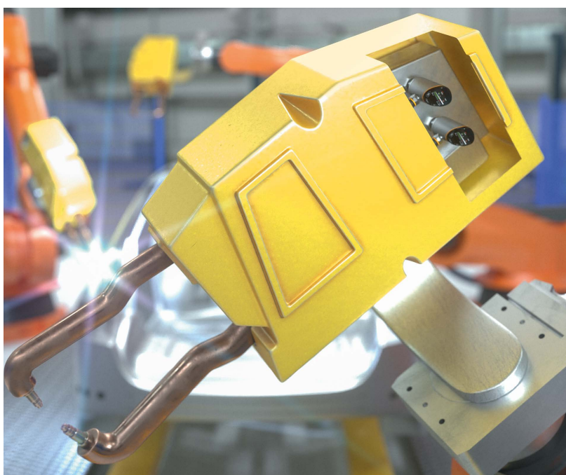
Monitoring the cooling circuit on welding clamps
